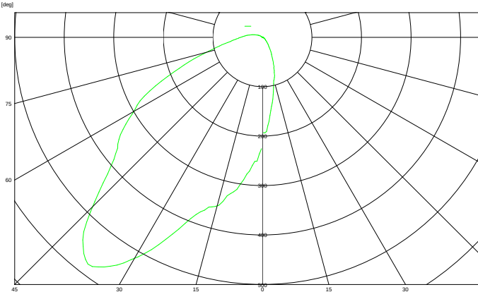
Illuminance angle, long side to ceiling
