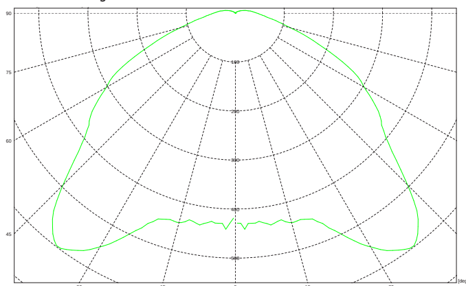
Illuminance angle
